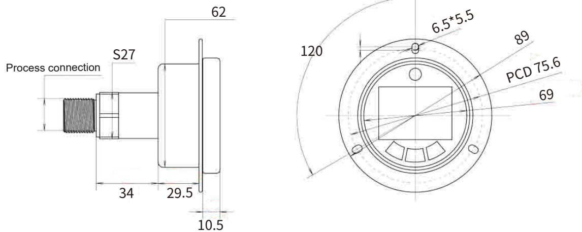
Back mount with flange 2.5"
